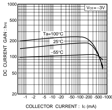
Fig.12 DC current gain vs. collector current (II)
